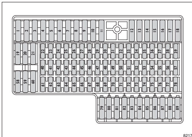
Fig. I-10 Facia fuseboard layout
