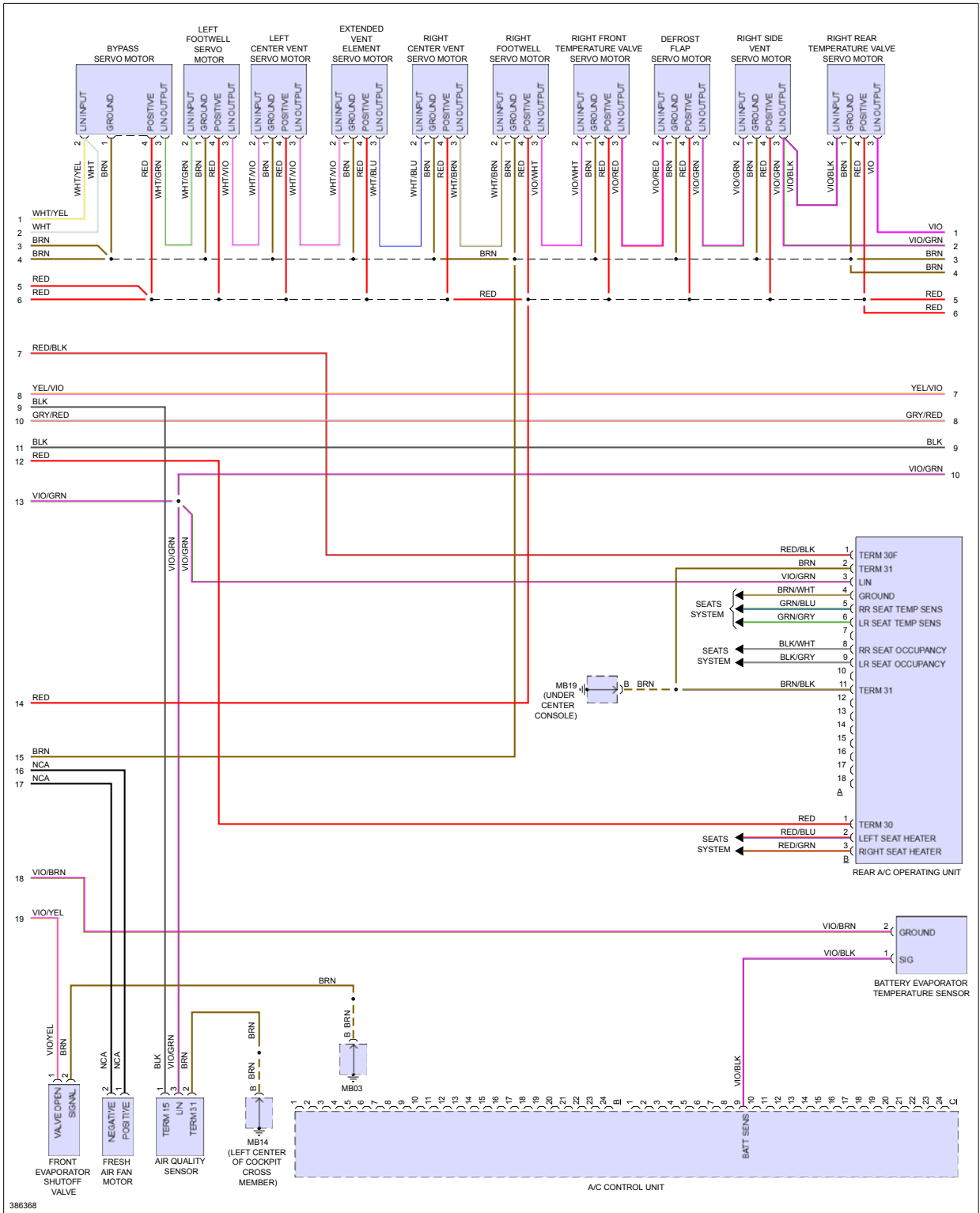
Fig 3: Automatic A/C Circuit, Except Hybrid (3 of 4)
