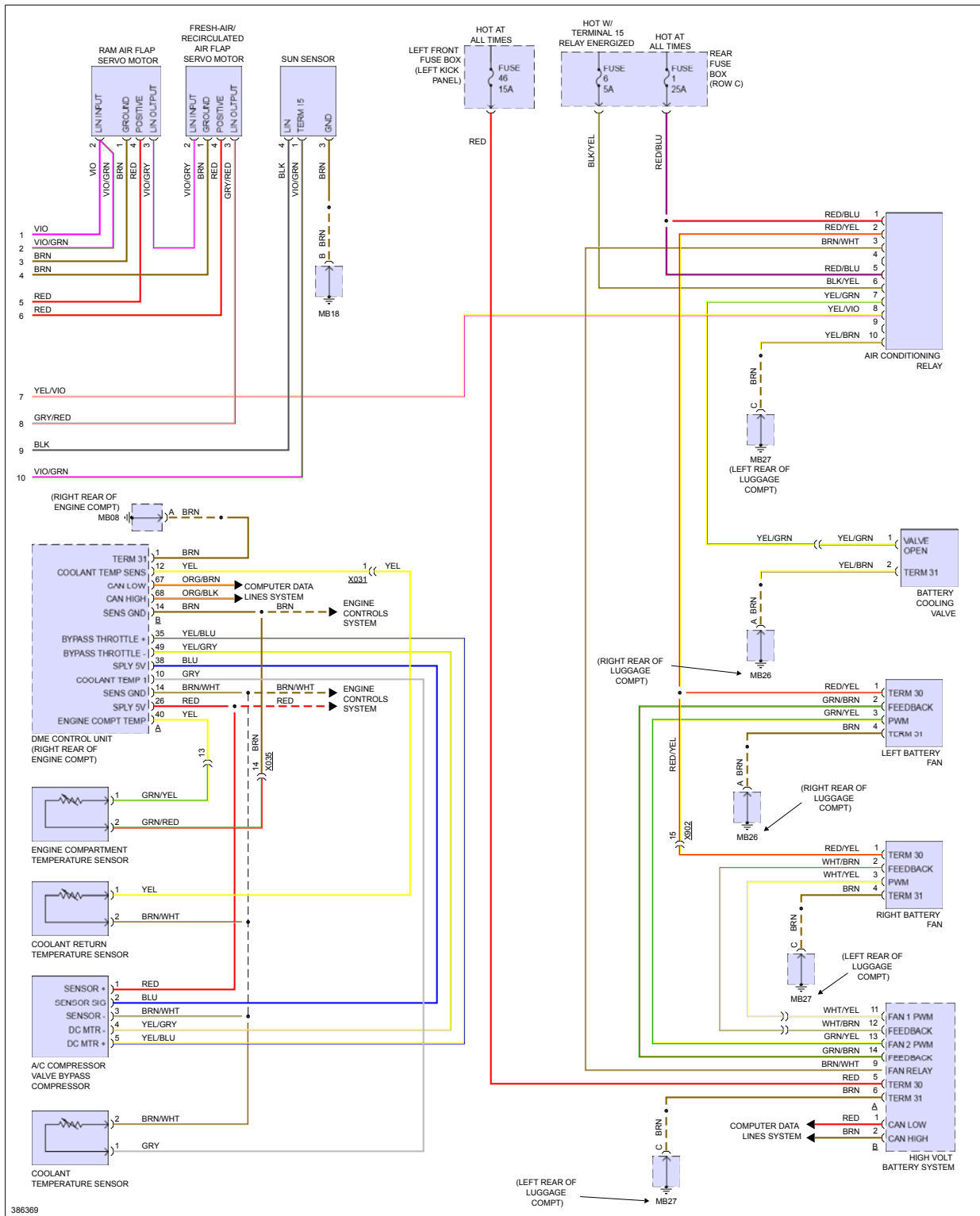
Fig 4: Automatic A/C Circuit, Except Hybrid (4 of 4)
