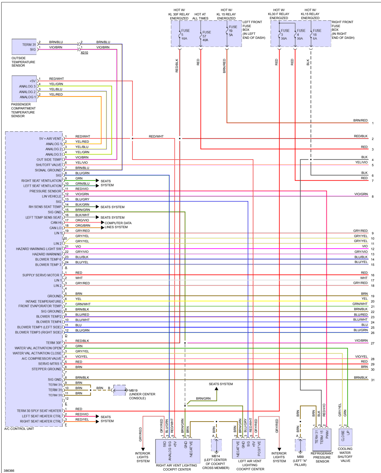
Fig 1: Automatic A/C Circuit, Except Hybrid (1 of 4)
